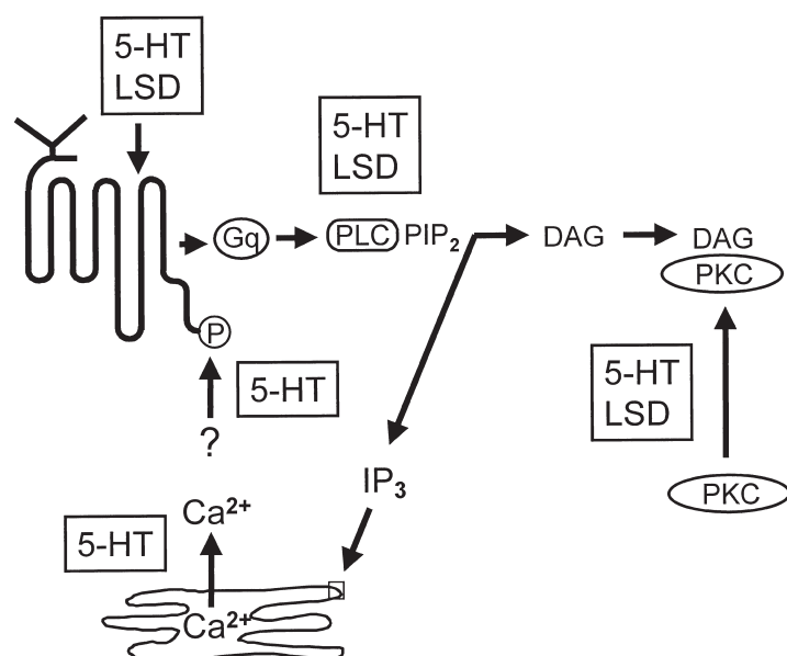
Figure 2. Schematic of 5-HT 2C receptor signal transduction and the sites of action of serotonin (5-HT) and lysergic acid diethylamide (LSD). LSD and serotonin are equipotent at promoting phosphoinositide hydrolysis through phospholipase C (PLC). LSD and serotonin also cause comparable translocation of immunoreactive protein kinase C (PKC) to the membrane. Whereas serotonin stimulates mobilization of intracellular calcium, LSD-mediated calcium release was not detected. LSD-mediated phosphorylation of the 5-HT 2C receptor was substantially lower than the serotonin signal.
